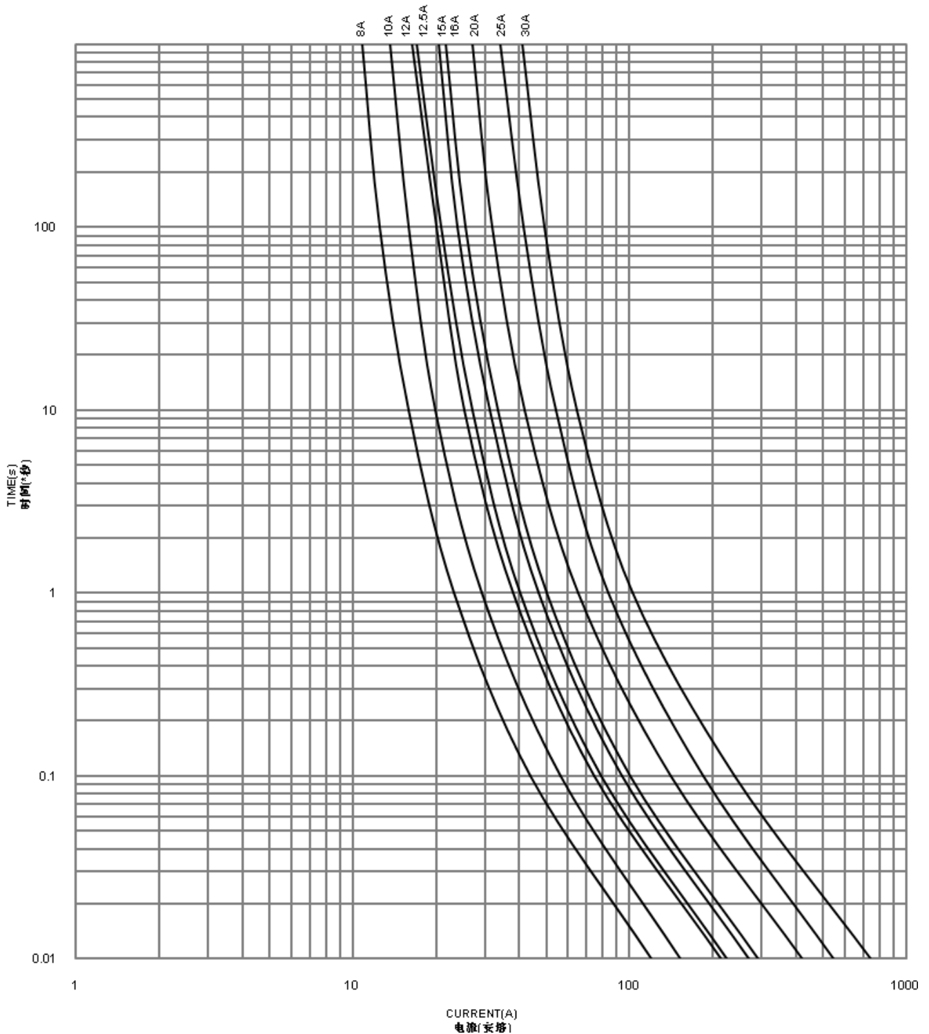
6TS Average I-T Characteristics Curve(For Reference Only) 6TS 平均电流-时间曲线图(仅供参考)
